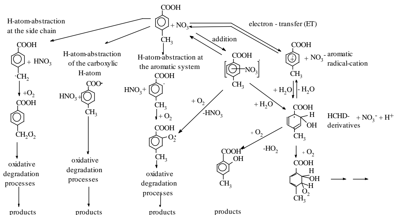
Fig. 1: Possible reaction pathways for the reaction of the NO 3 · radical with aromatic compounds in aqueous solution.
