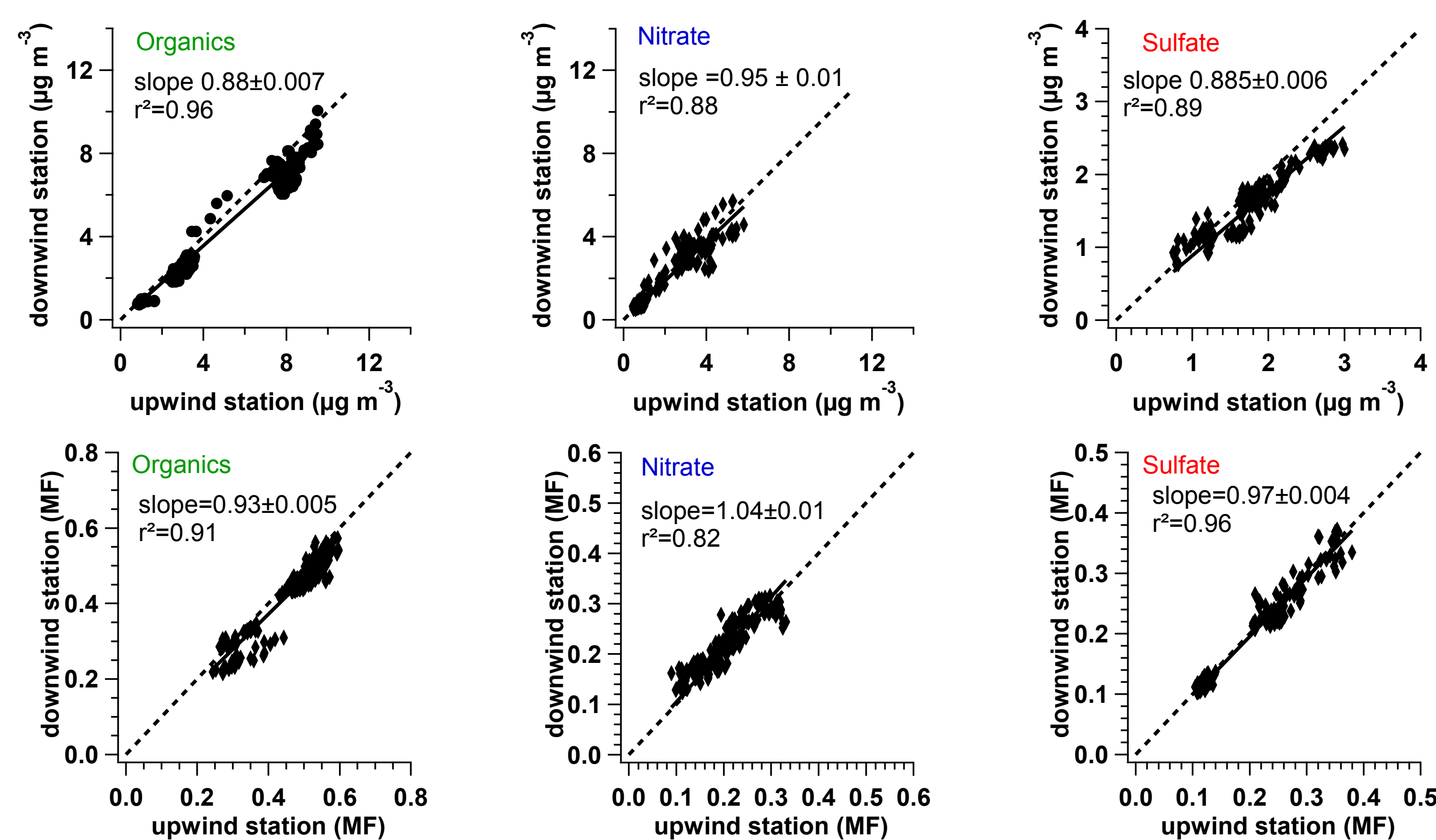
Figure 3: Mass concentration (upper panel) and mass fraction (lower panel) of organics, nitrate and sulfate measured downwind and upwind of the mountain during dry-overflow (NCE)
