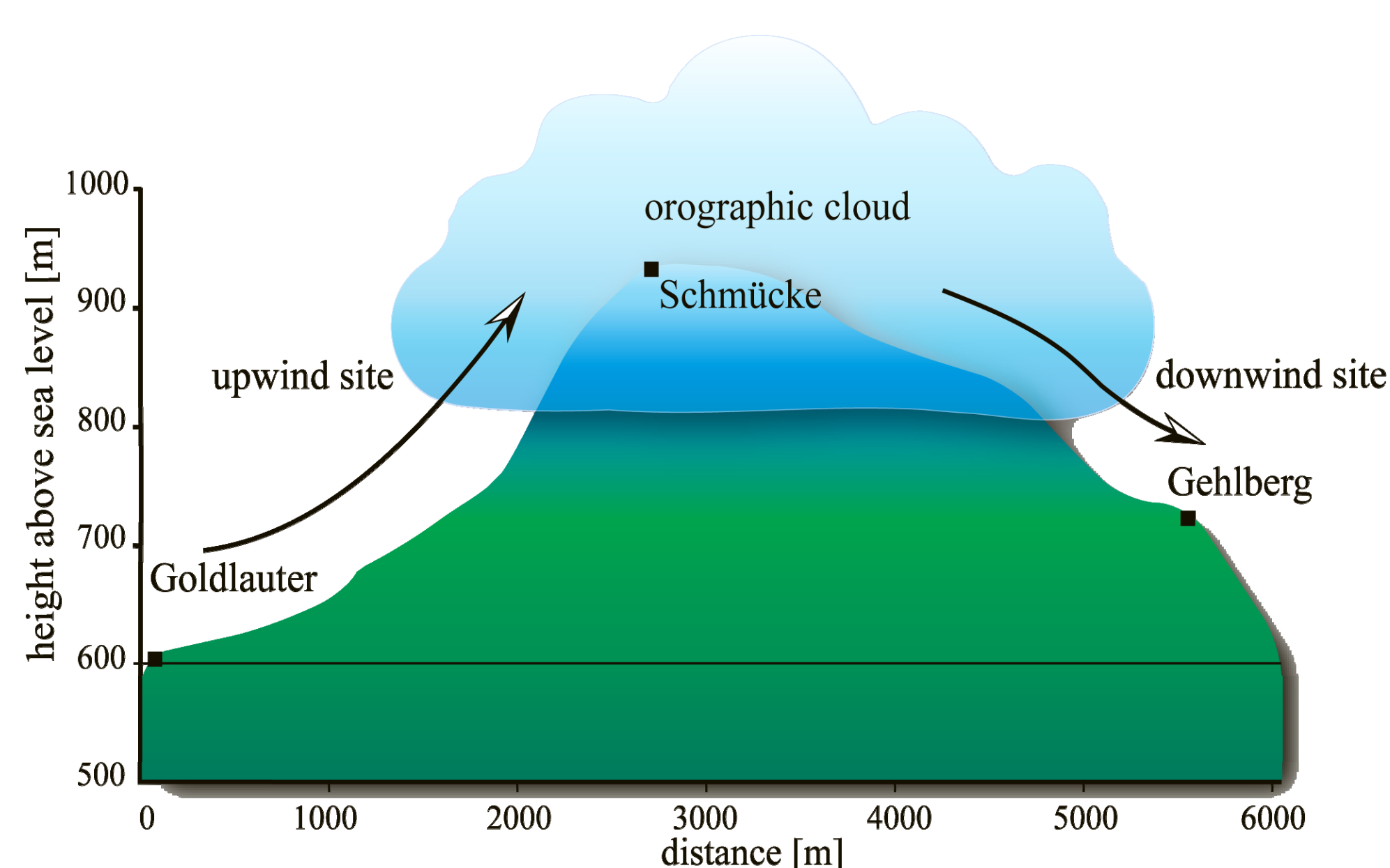
Figure 1: Scheme of the HCCT-2012 sampling sites and the general philosophy of cloud passage experiment HCCT-2010
