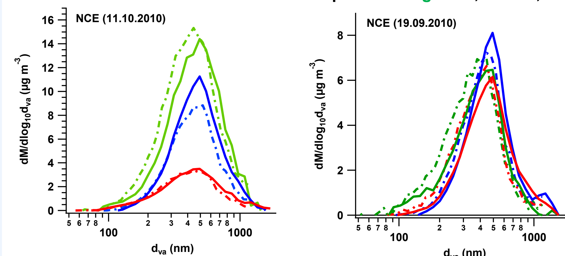
Figure 5: Average chemical size distribution for different FCE and NCE.
