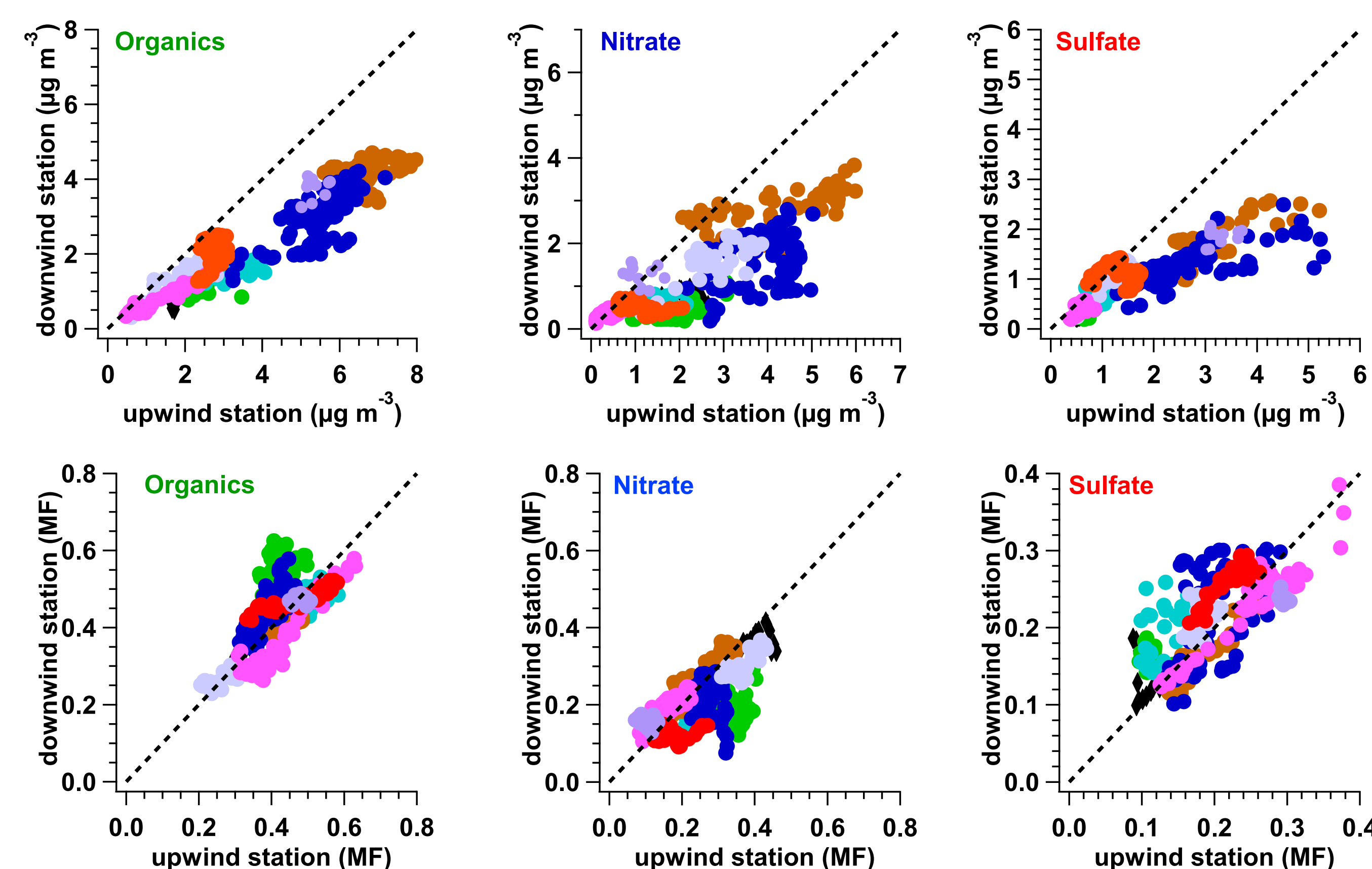
Figure 3: comparison of the mass concentration and mass fraction during the different cloud events (FCE)
