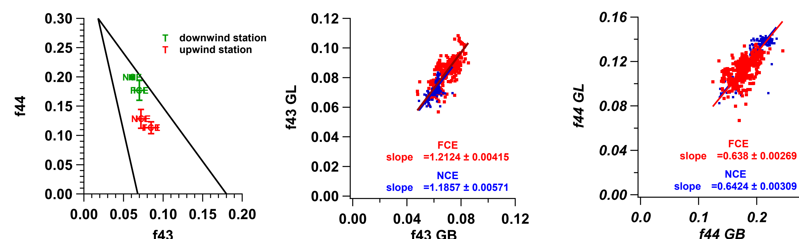
Figure 4: Change in organic contribution of m/z 44 and 43 during dry overflow and cloud events
